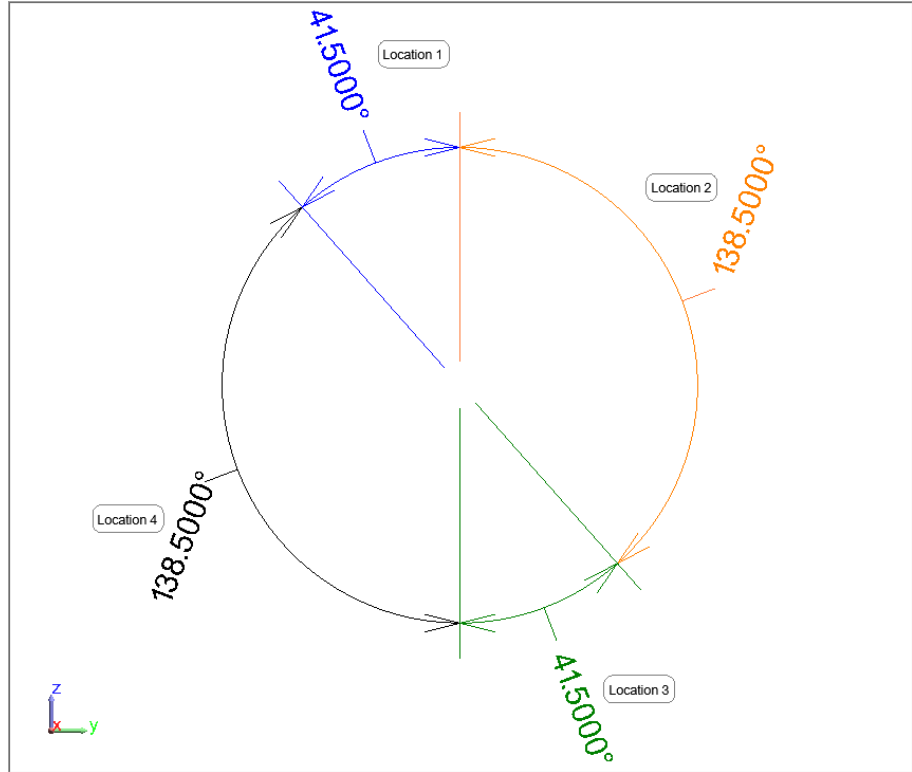
Figure 27-32. Angular quadrants
