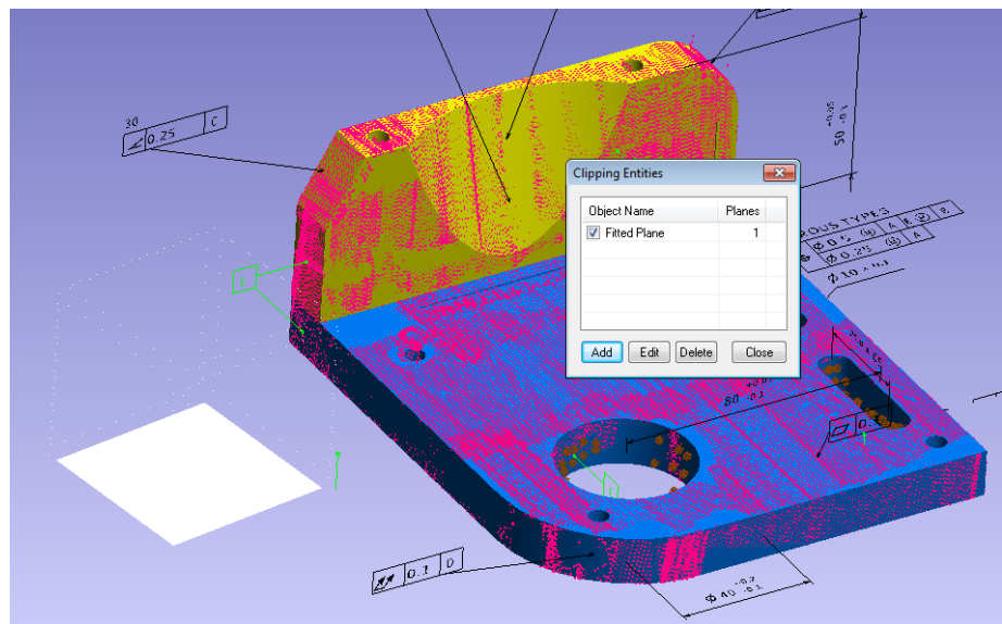
Figure 9-18. Clipping Plane
