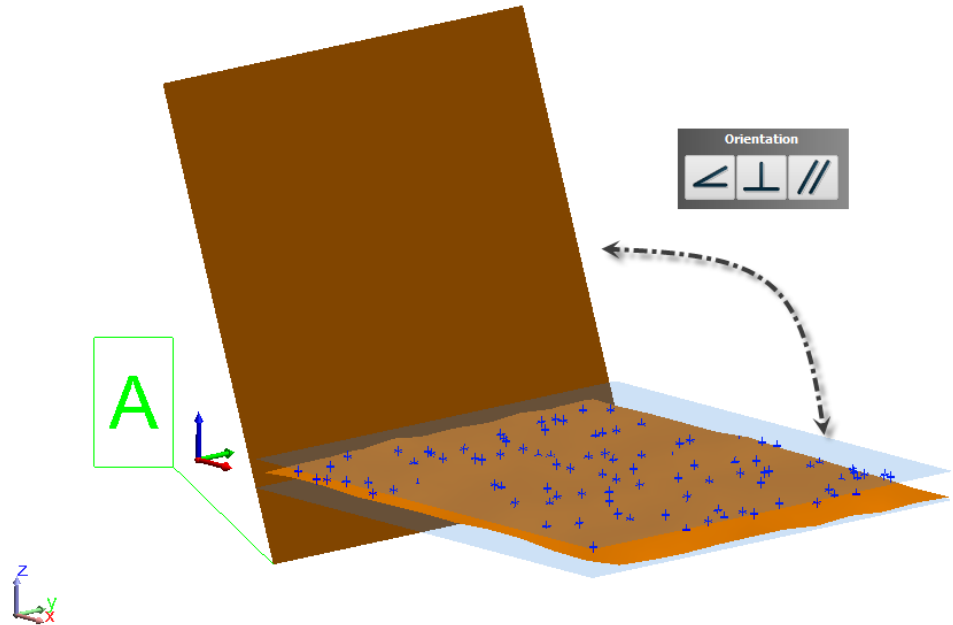
Figure 26-35. Planar Evaluation
