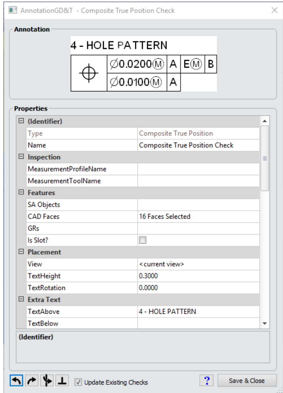
Figure 27-10. Example Annotations Properties Dialog.
