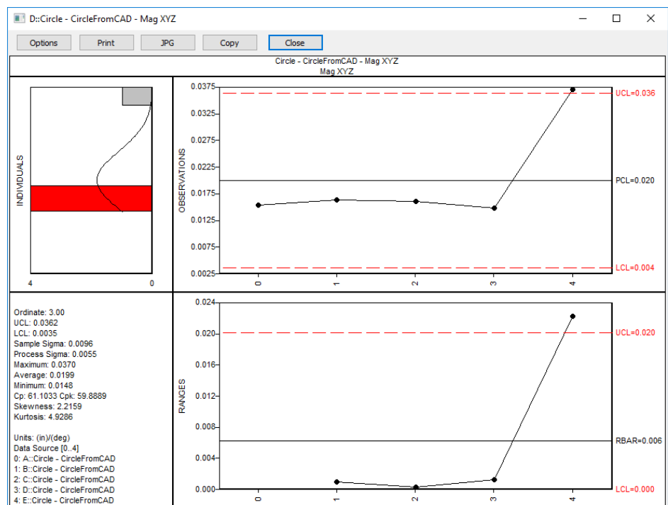
Figure 28-95. Example circle position SPC chart
