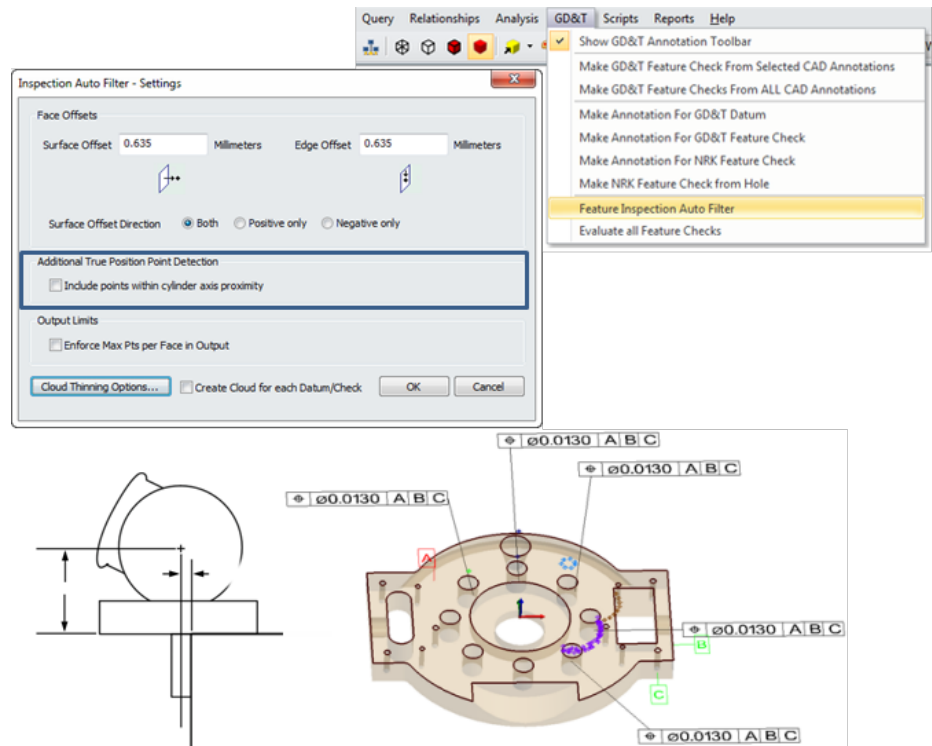
Figure 27-50. True Position Point Detection
