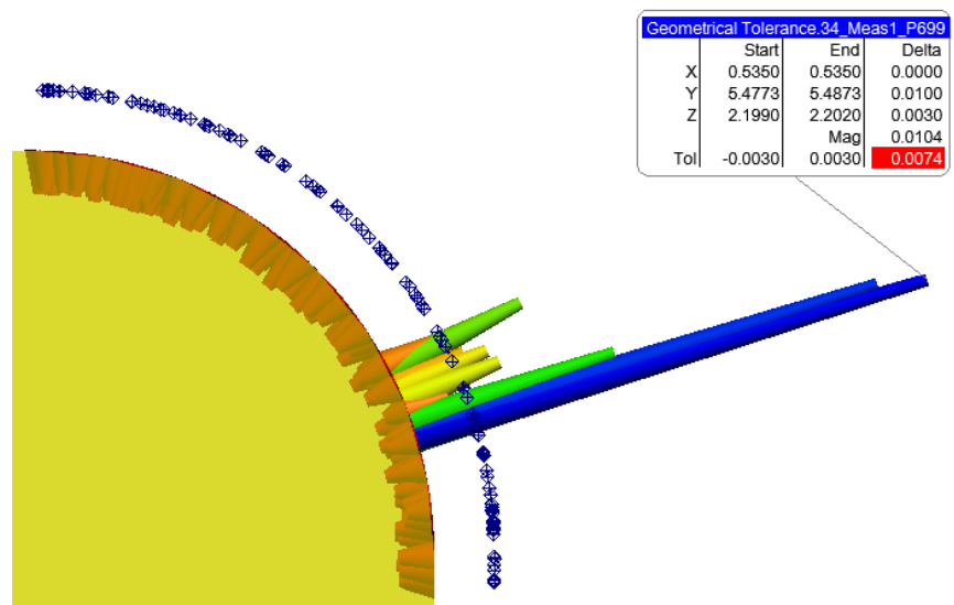
Figure 28-88. A vector callout.
