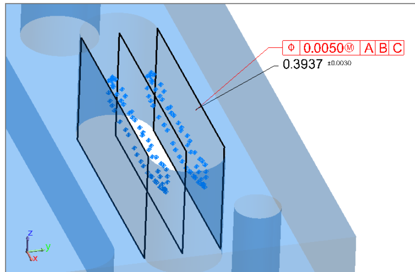
Figure 27-27. Mid Plane Evaluation of a slot.
