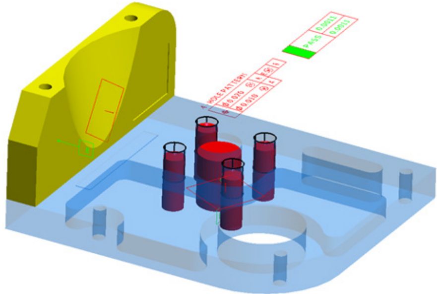
Figure 27-24. Resulting geometry from enabling the Feature Creation check boxes on a Composite True Position check.
