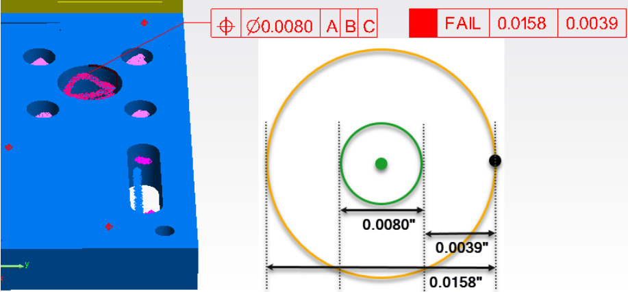
Figure 27-59. Reported values for a position check showing the Distance Out of Tolerance value.
