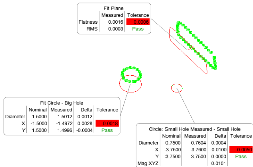
Figure 28-77. Geometry relationship callouts in the graphical view.
