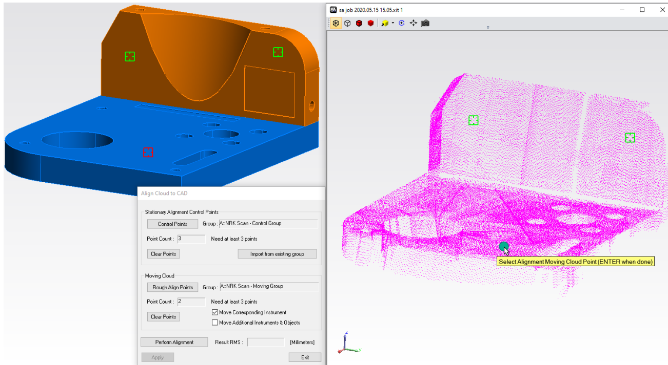
Figure 25-58. Align Cloud to CAD windows and arrangement.
