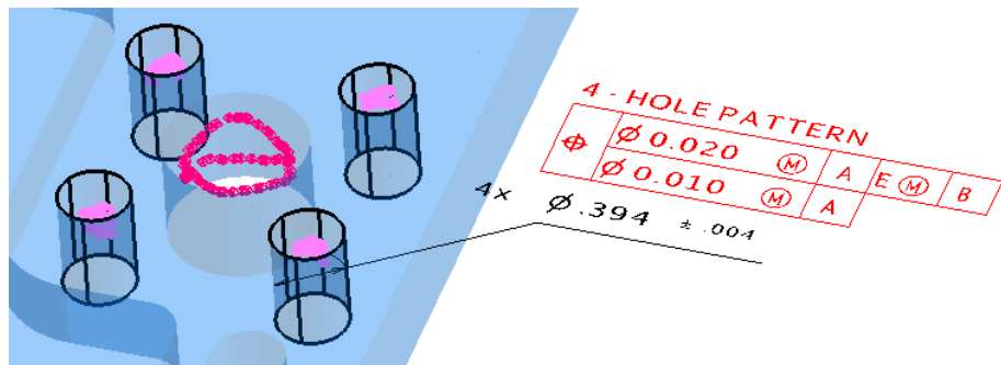
Figure 27-45. Composite True Position Check
