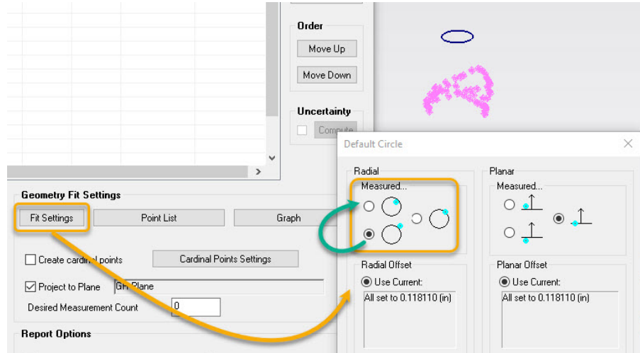
Figure 25-33. Changing the Geometry fit settings from pin to hole
