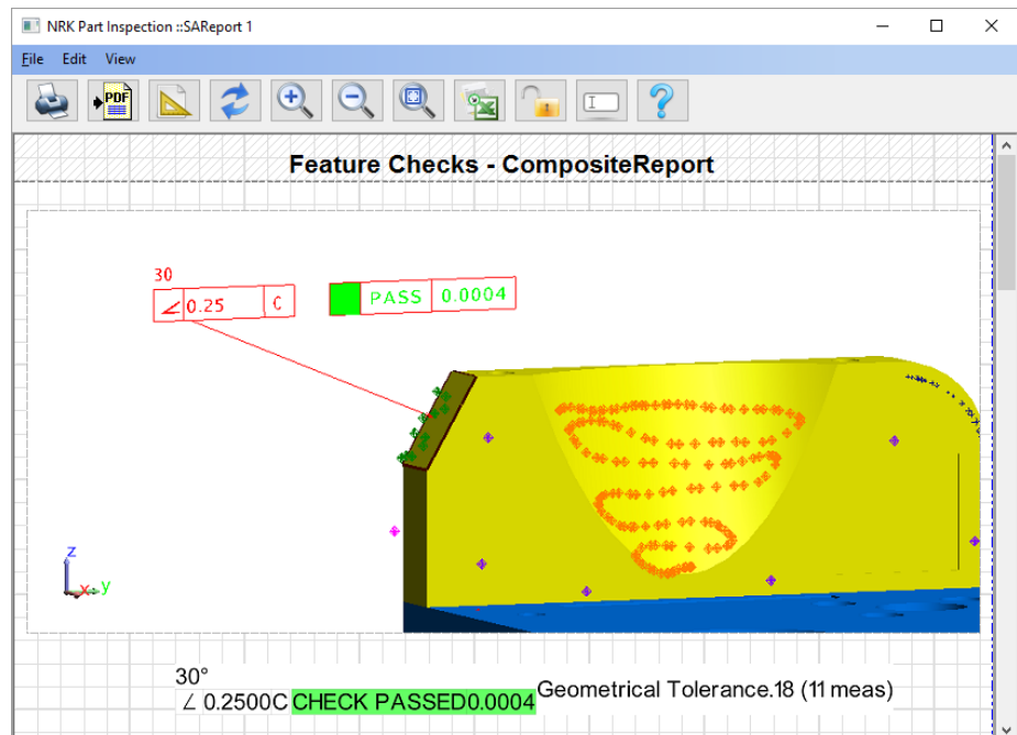
Figure 27-60. Composite Quick Report Example
