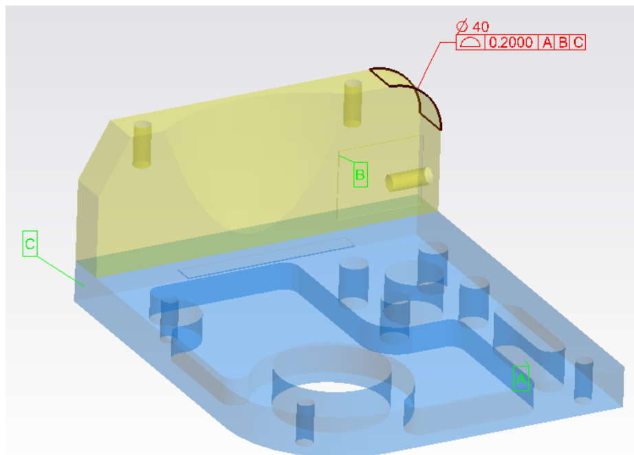
Figure 27-49. Show Only Active Feature Check Option Enabled
