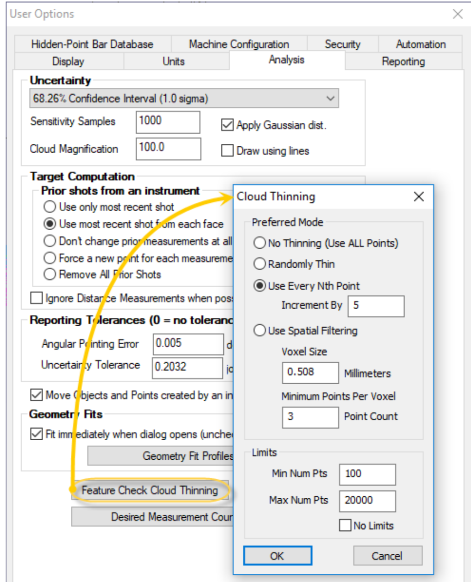
Figure 27-29. Cloud Thinning Controls
