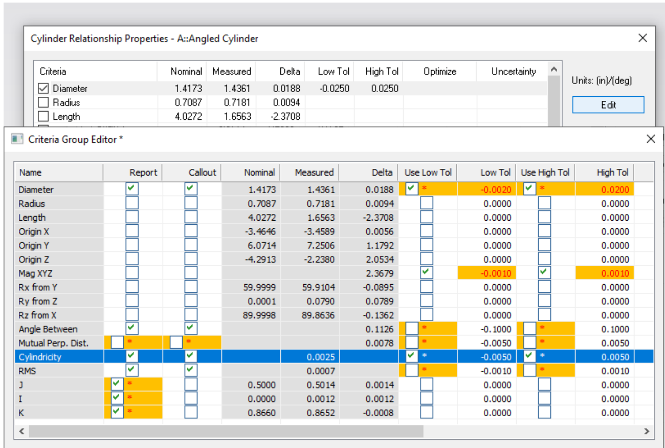
Figure 15-22. Criteria Group Editor.
