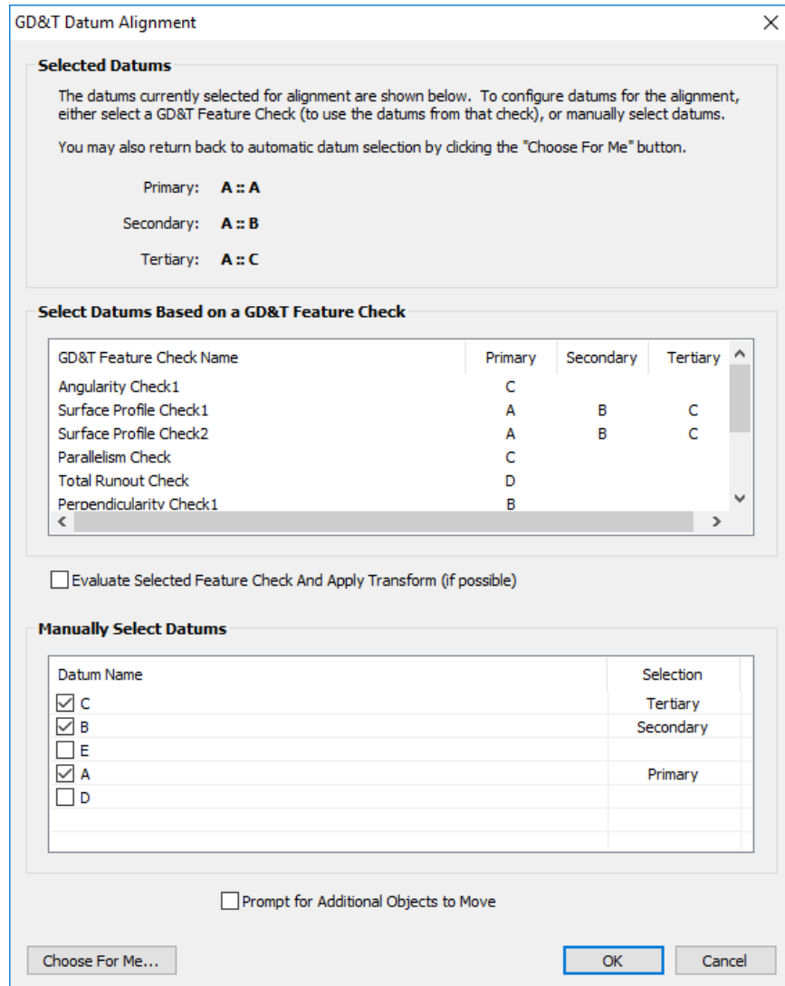
Figure 27-19. Datum Align Tool
