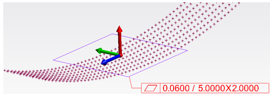
Figure 27-36. The Z-axis of the selected SA object is used to define the Length direction in a per unit area flatness check.
