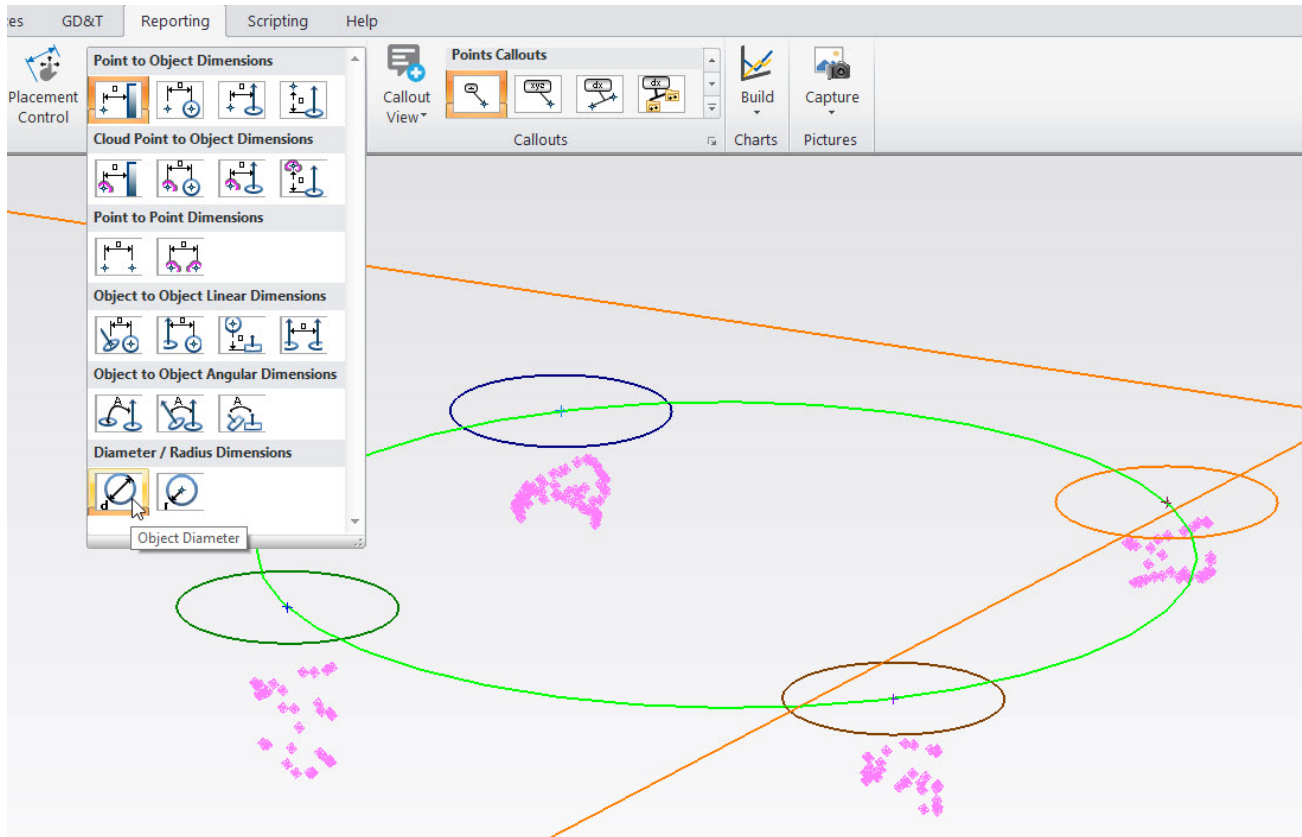
Figure 25-39. Adding a diameter dimension to the circle from multiple circles
