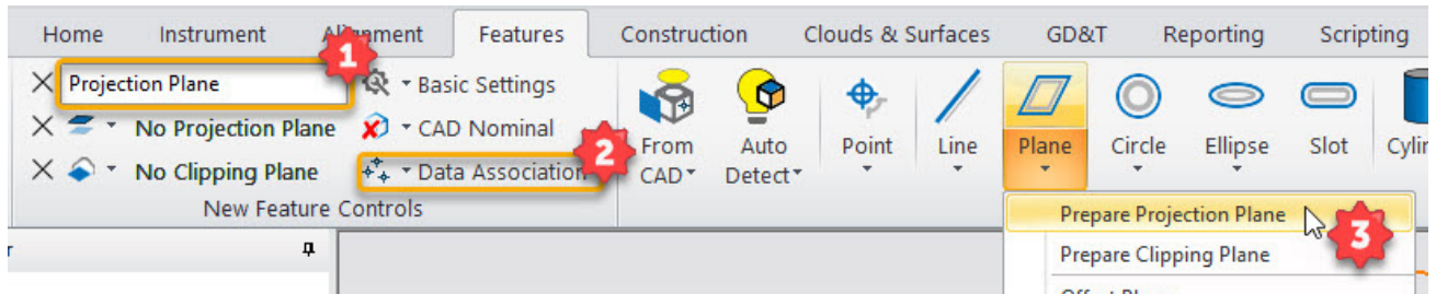
Figure 25-31. Steps to build a projection plane
