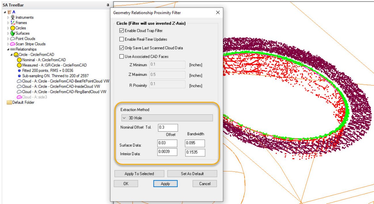
Figure 26-55. 3D Hole extraction which is using a Scan Stripe Cloud as an input and builds 3 results. The local plane, the interior data, and a projected set of data used for the circle fit.
