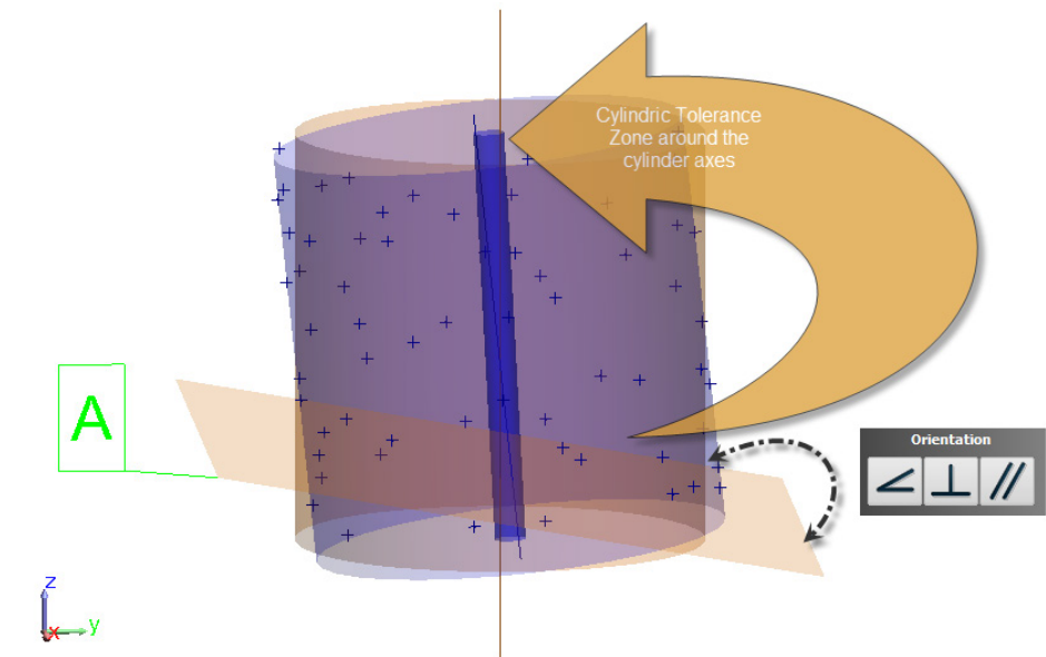
Figure 27-38. Axial Evaluation
