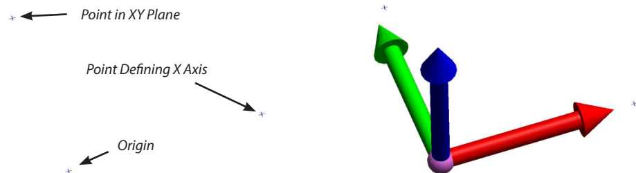
Figure 9-11. Points used to define a 3-2-1 frame (left) and the resulting constructed frame (right).
