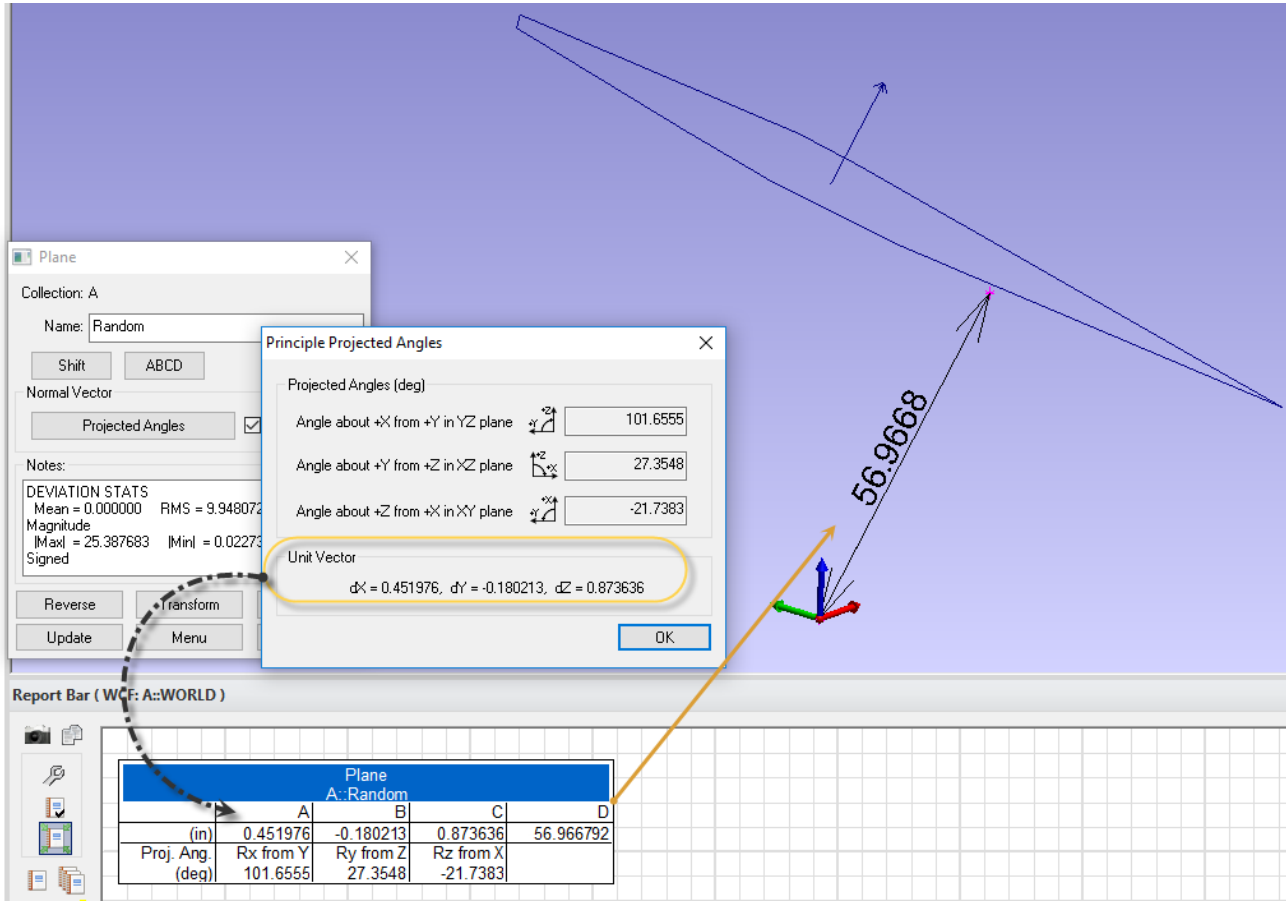
Figure 10-5. ABCD Definition
