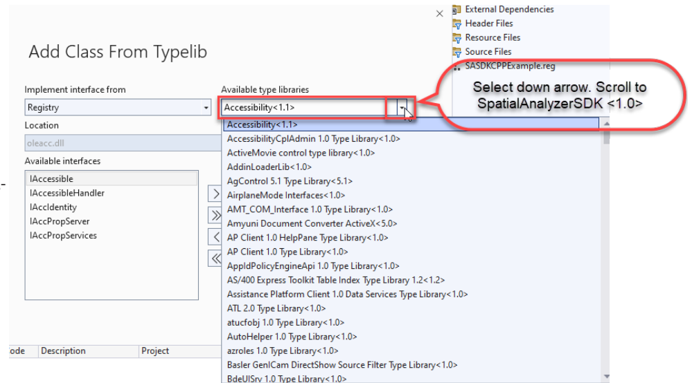
Figure 33-14. Selecting SpatialAnalyzerSDK <1.0>
