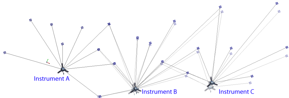
Figure 30-3. Positional errors resulting from leap-frogging an instrument along a length.
