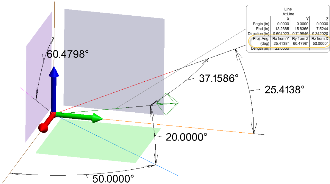
Figure 9-6. Visualizing Projected Angles for a line or axis
