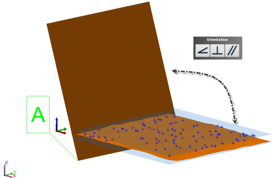
Figure 26-37. Planar Evaluation
