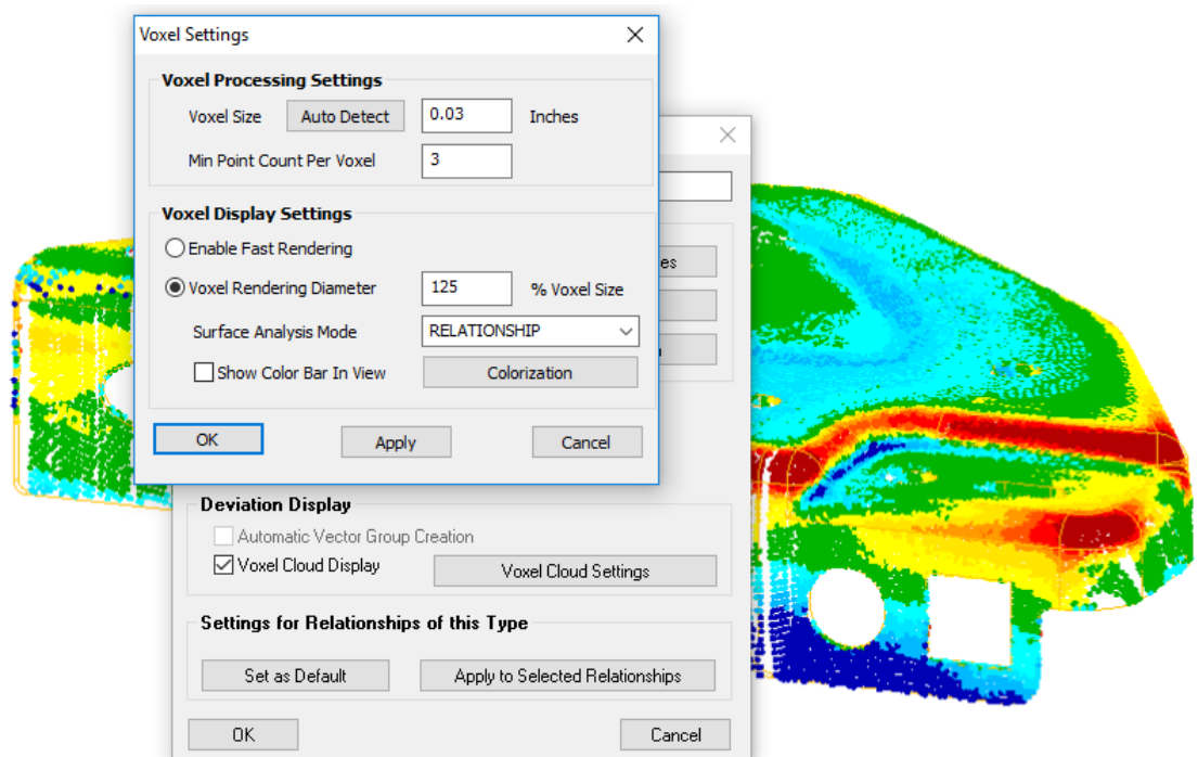
Figure 9-20. Voxel Settings for Surface Deviation Display
