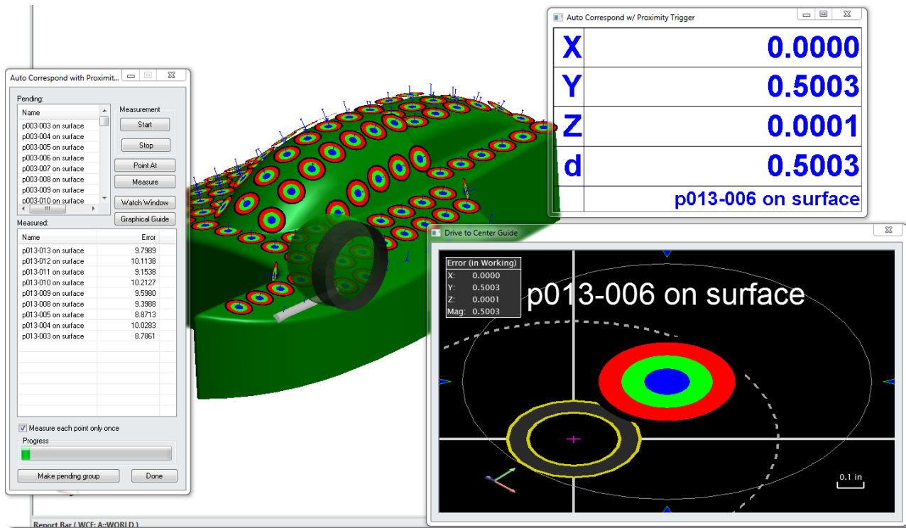
Figure 13-35. Proximity Measured Points in progress
