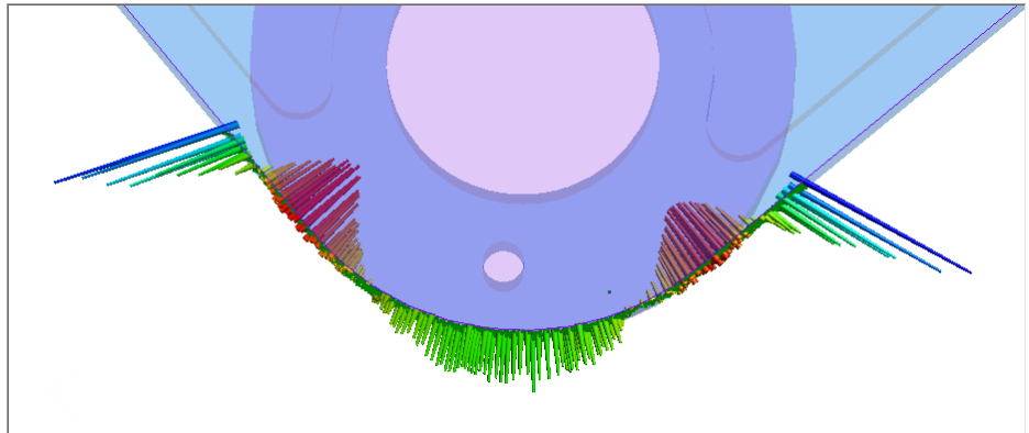
Figure 9-50. Partial cylinder proximity filter problem. Showing the need to save CAD face information.
