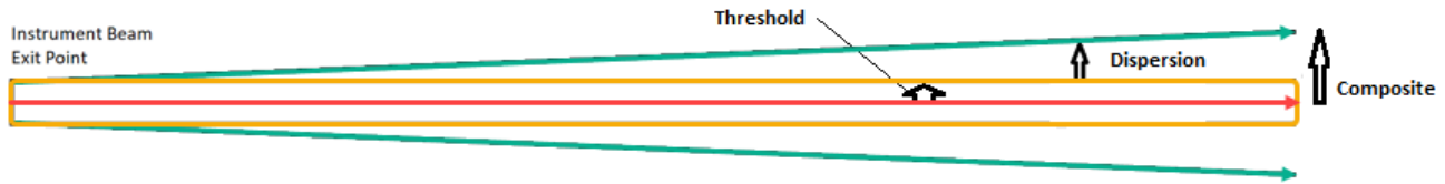
Figure 28-10. Error Dispersion Model for EDM Uncertainty
