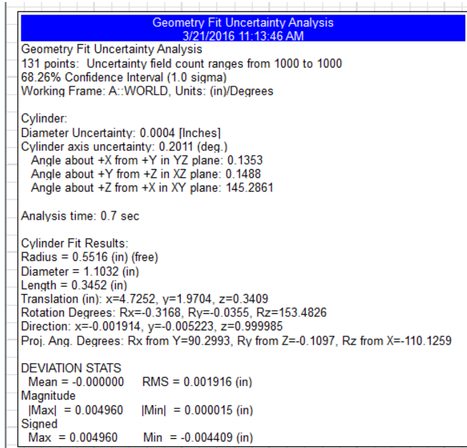
Figure 28-21. Cylinder Fit Event
