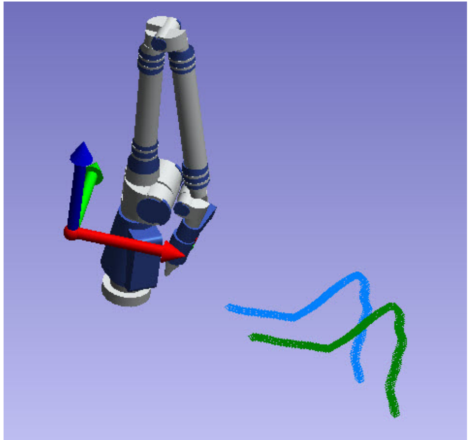
Figure 13-39. Scanning a path to locate the arm. A path along 3 axes of a fame works well.
