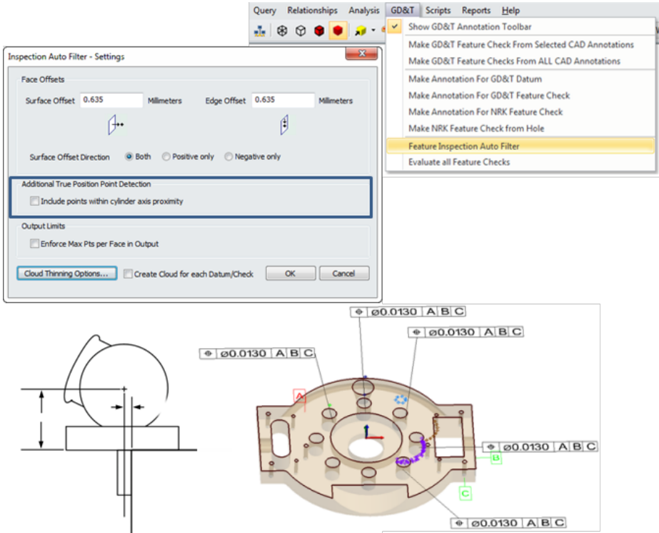
Figure 26-50. True Position Point Detection
