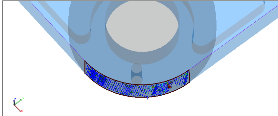
Figure 9-52. Properly filtered data using the associated CAD faces and resulting vectors.
