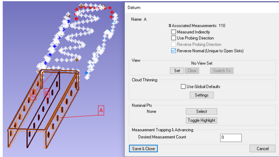
Figure 26-20. Incorrect alignment resulting from a datum being flipped. This can be fixed in the Datum properties.
