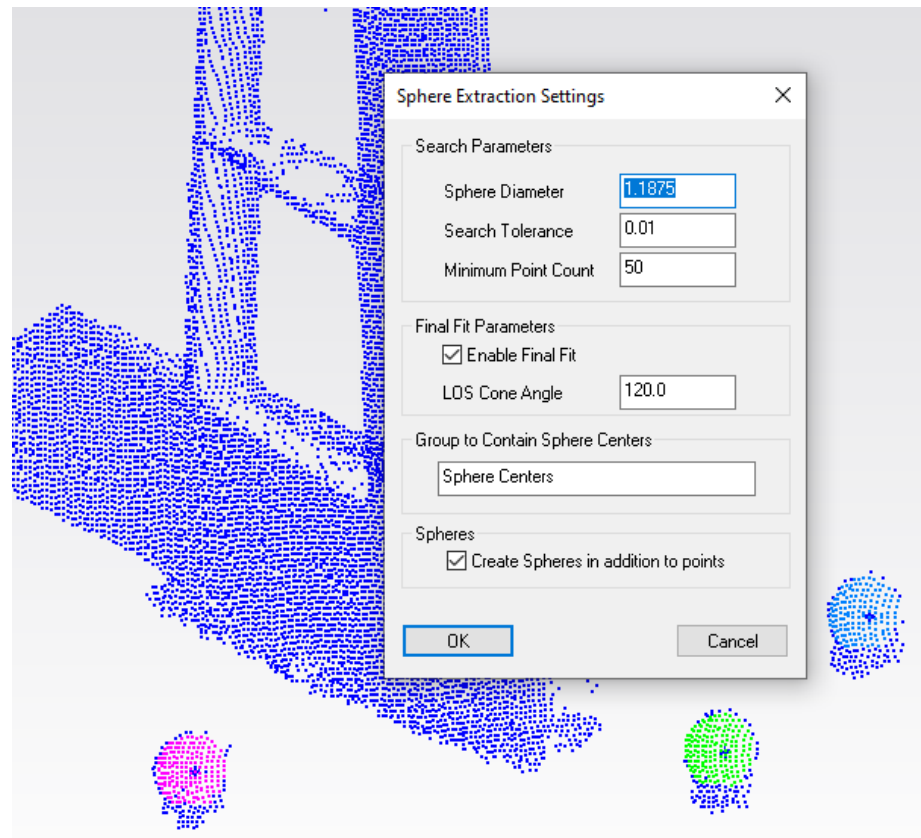
Figure 9-40. Registration sphere centers have been automatically extracted from this scan.
