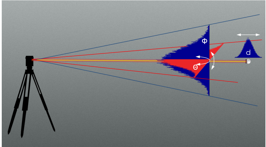
Figure 28-8. Component Instrument Uncertainty for a Tracker
