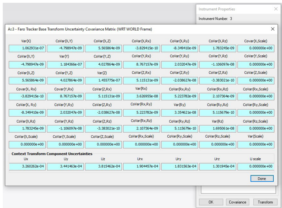
Figure 29-34. Example Instrument Covariance
