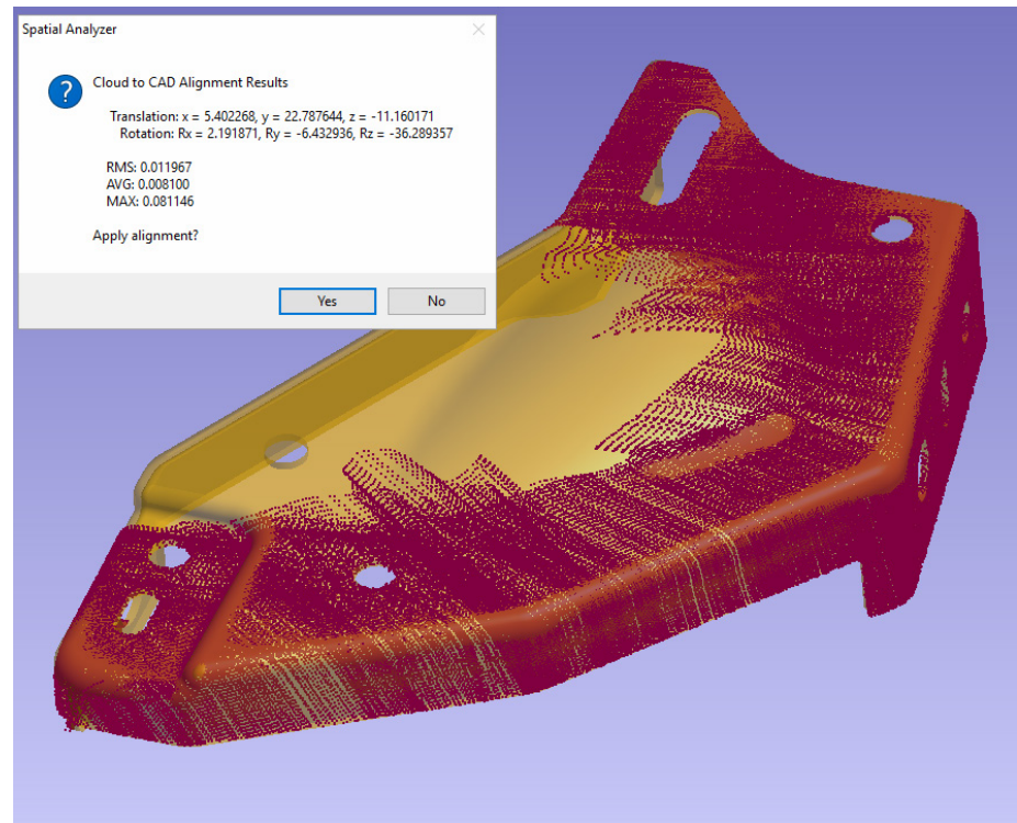
Figure 9-44. Align to CAD
