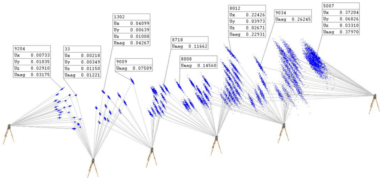
Figure 29-25. Example of error expansion from a single fixed instrument
