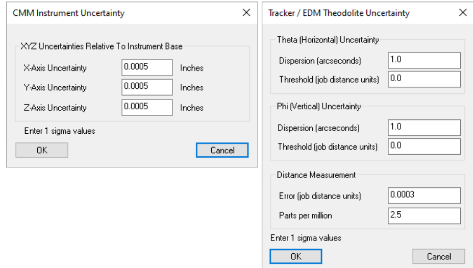
Figure 28-7. Instrument Uncertainty Variables
