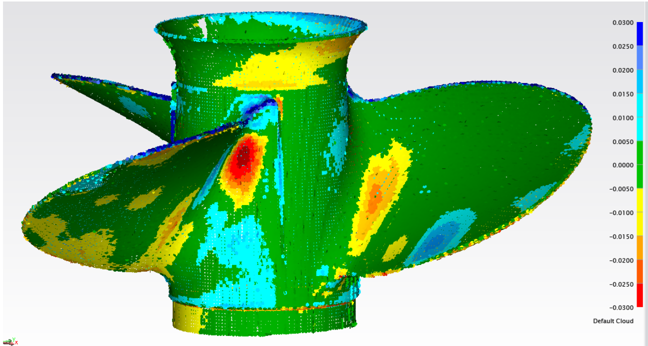
Figure 9-15. Voxel display of deviations from a scan of a propeller.
